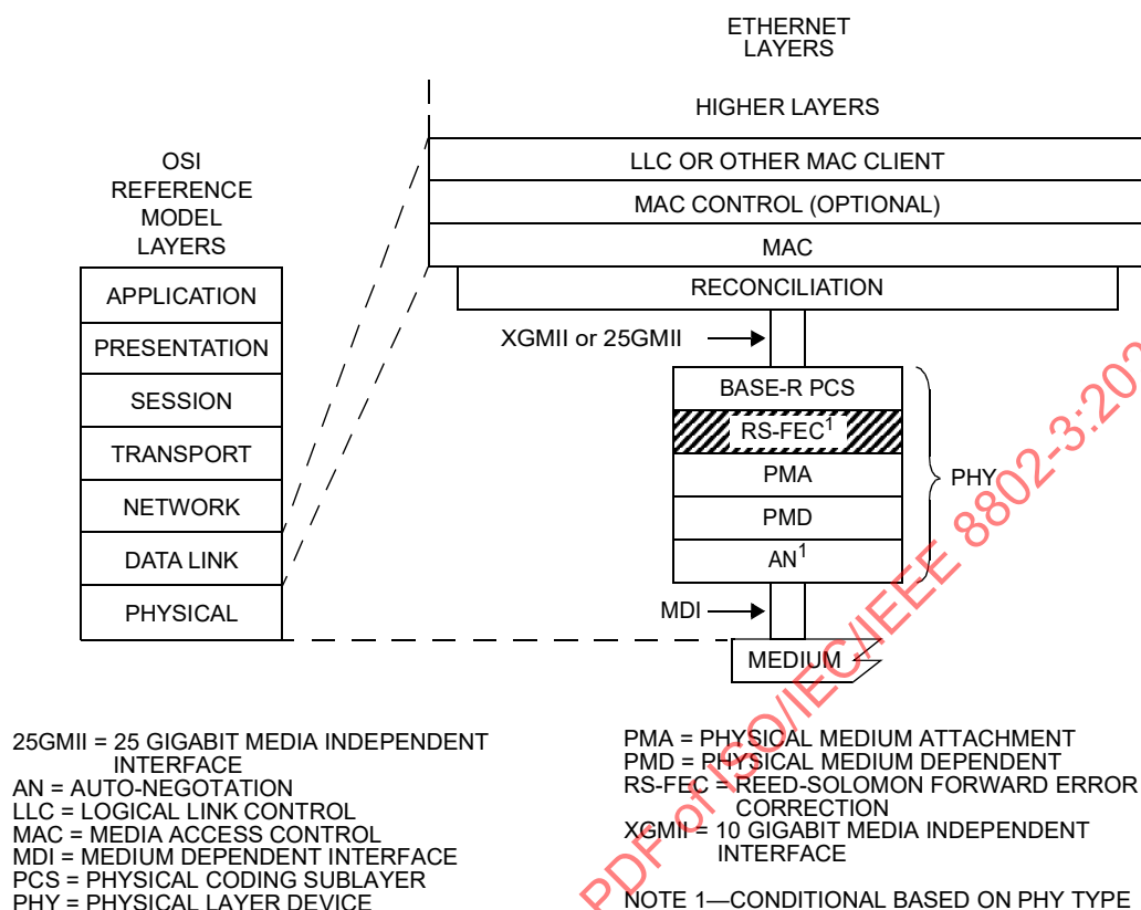
Figure 108–1—10GBASE-R and 25GBASE-R RS-FEC relationship to the ISO/IEC Open Systems Interconnection (OSI) reference model and the IEEE 802.3 Ethernet model
