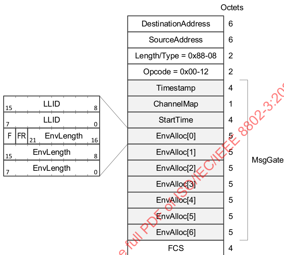
Figure 144–12—GATE MPCPDU
