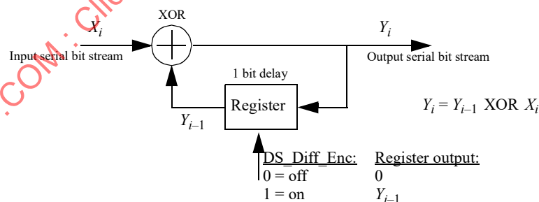
Figure 142–18—Differential encoding
