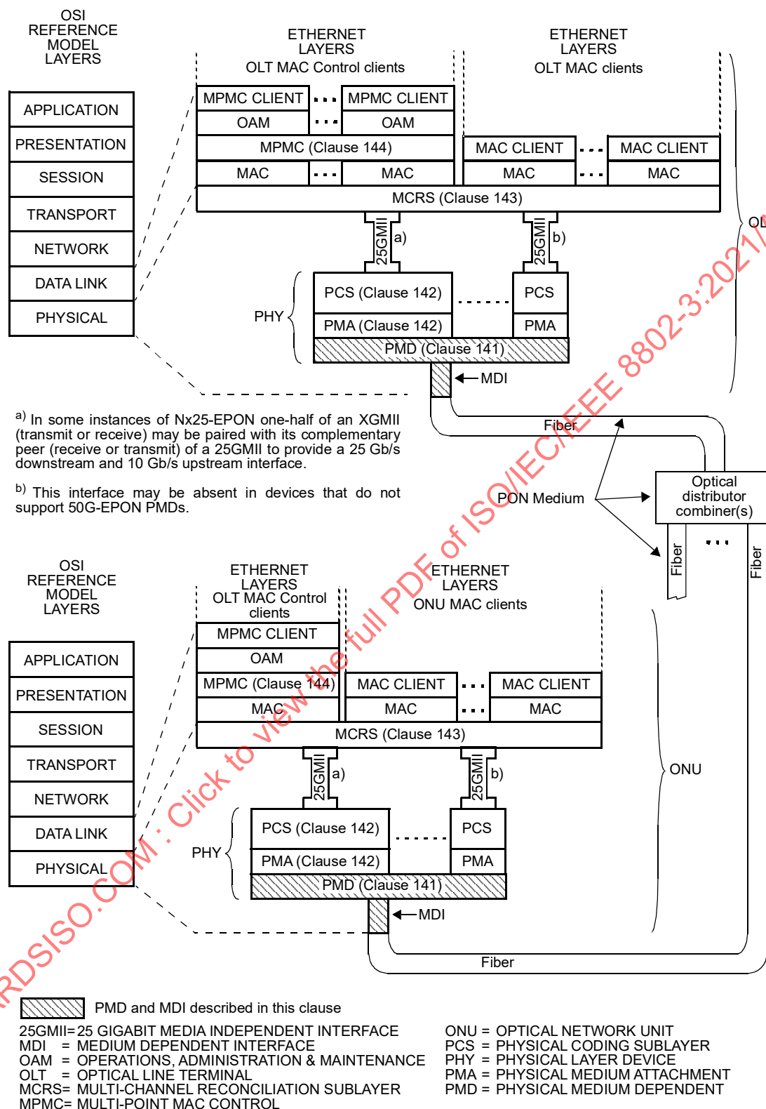
Figure 141-1—Relationship of Nx25G-EPON P2MP PMD to the ISO/IEC OSI reference model and the IEEE 802.3 Ethernet model
