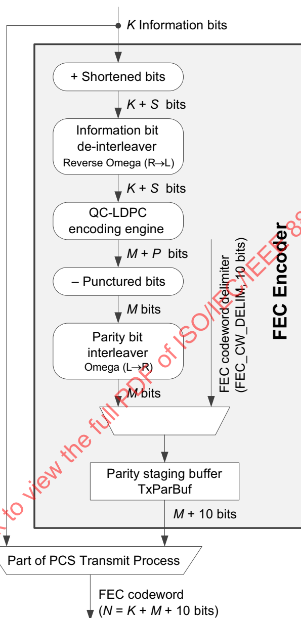
Figure 142–5—FEC encoder
