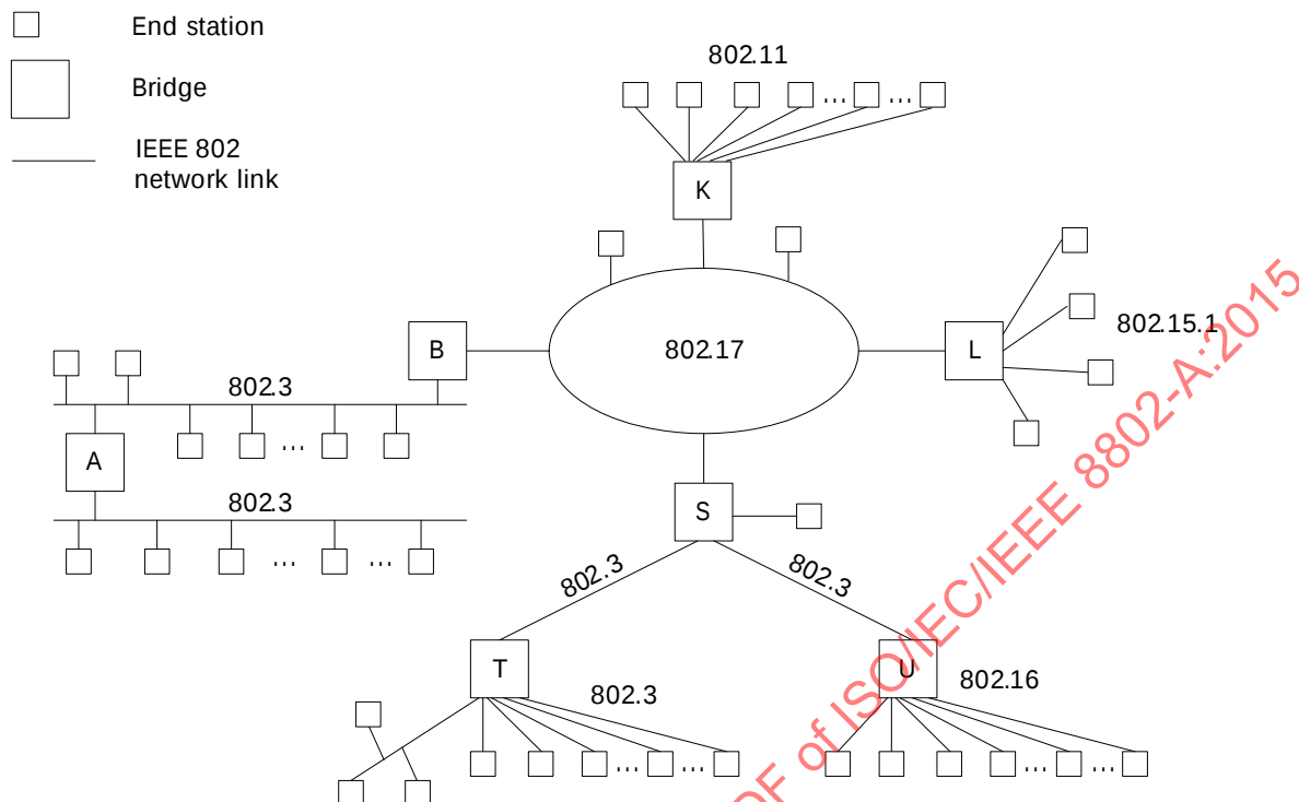
Figure 8—An example of a bridged IEEE 802 network
