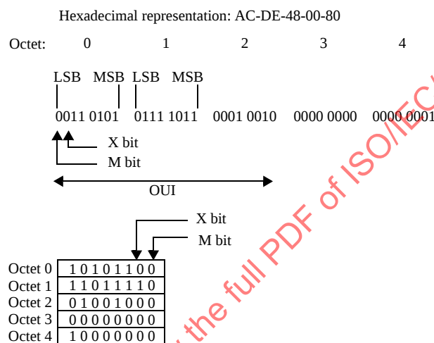
Figure 17—SNAP identifier
