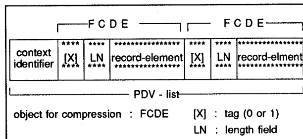
Figure 5 - INTAP-TS1 compression method
