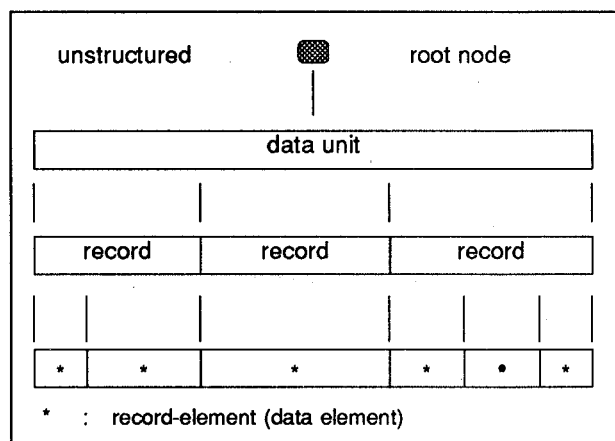
Figure 1 - INTAP-1 document type structure
