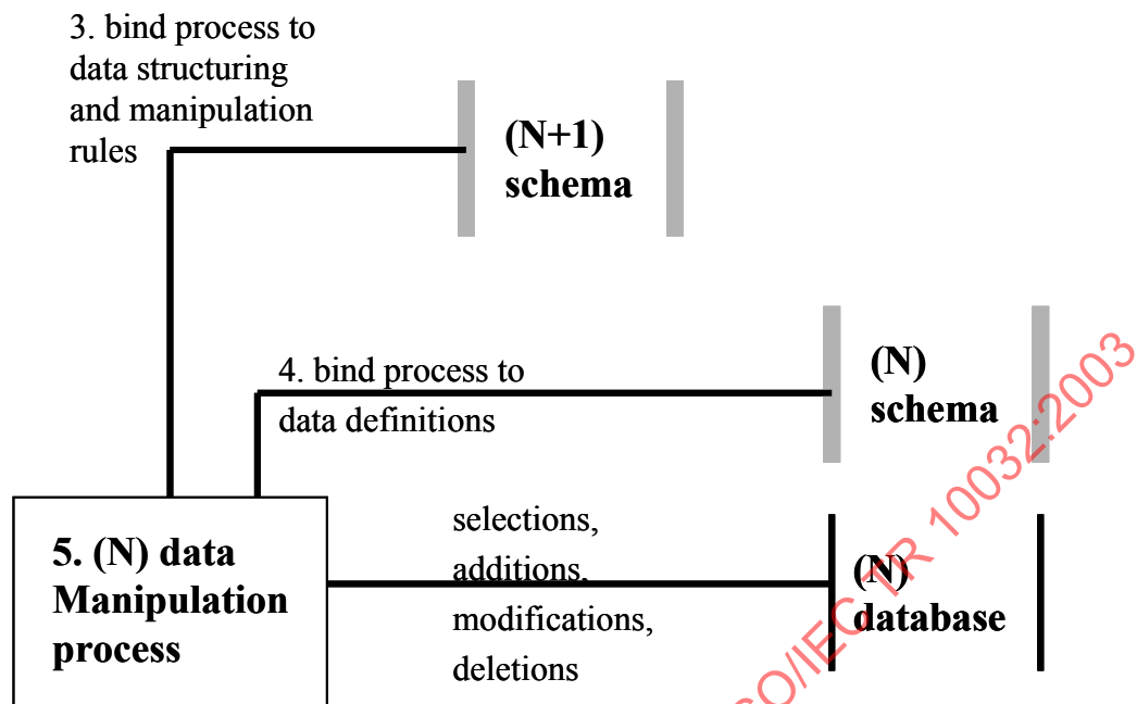
Figure 6 — Binding and data manipulation
