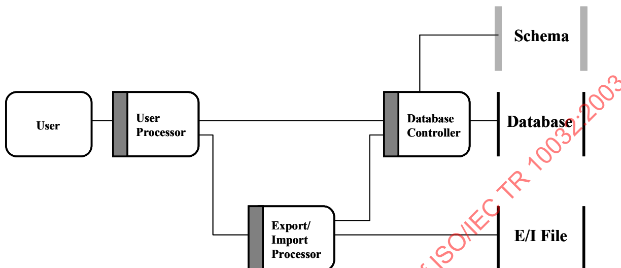
Figure 12 — The model of export/import
