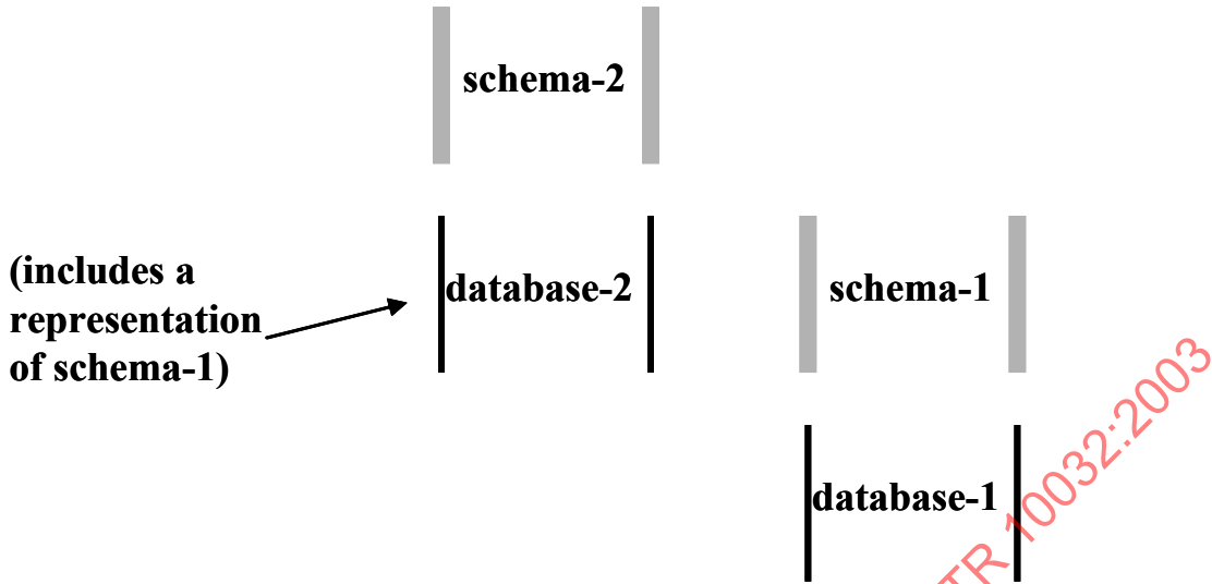
Figure 3 — Interlocking level pair
