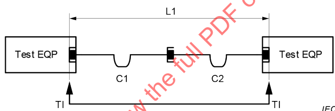
Figure 3 – Two-segments, three-connections, E2E link
