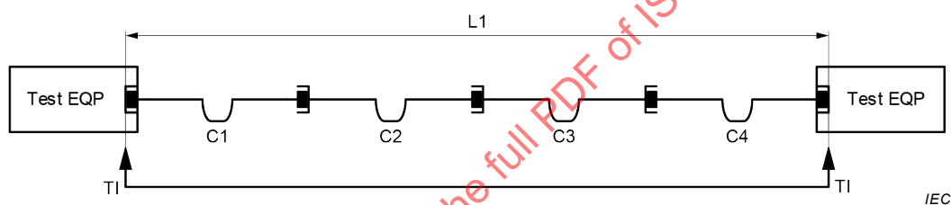
Figure 8 – Four-segments, five-connections, E2E link
