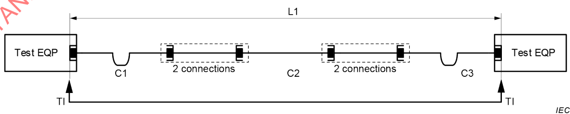
Figure 5 – Three-segments, six-connections, E2E link
