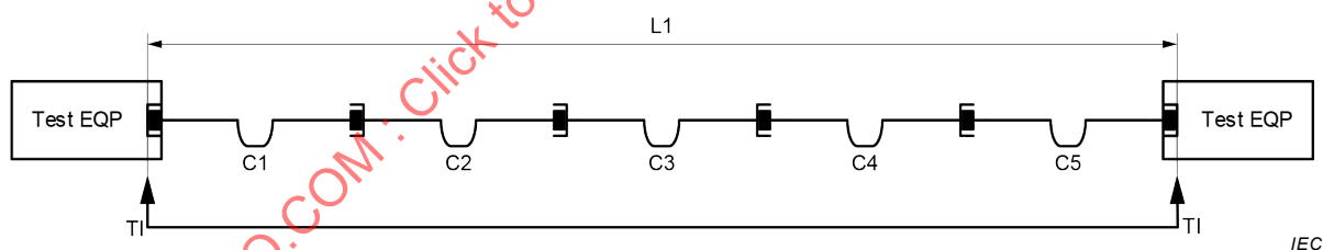
Figure 9 – Five-segments, six-connections, E2E link
