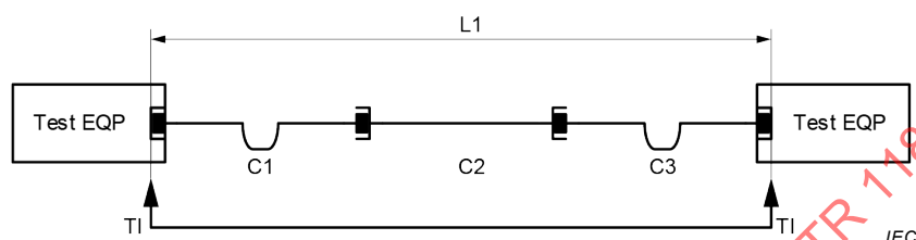
Figure 7 – Three-segments, four-connections, E2E link
