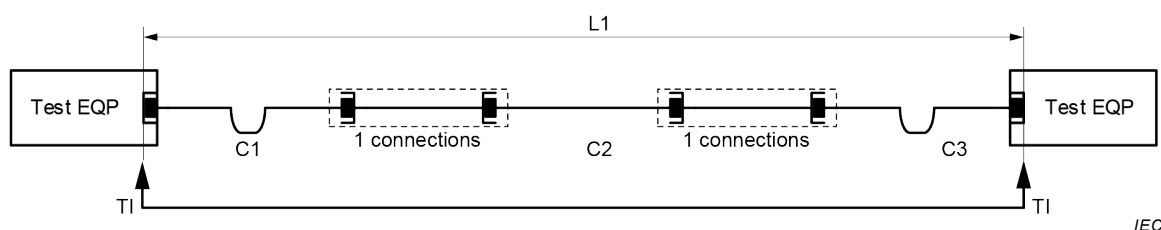
Figure 6 – Three-segments, four-connections, E2E link
