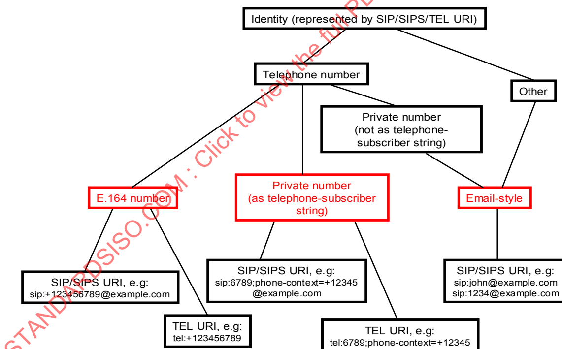
Figure 1 — Relationships between different forms of SIP and TEL URIs
