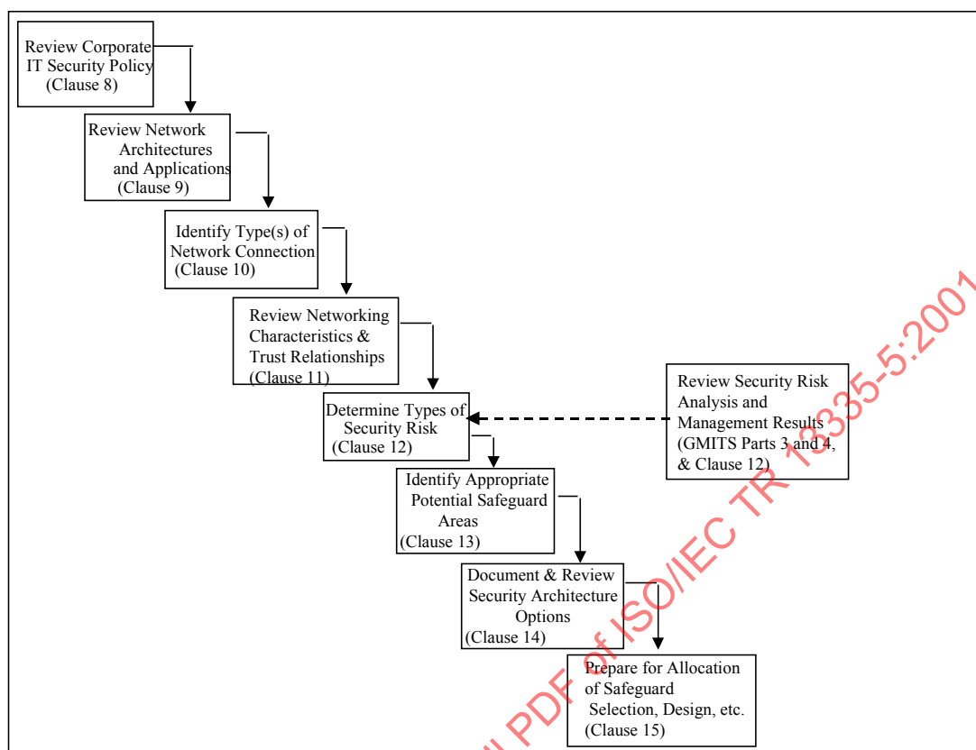
Figure 1: Process for the Identification and Analysis of Communications Related Factors Leading to the Establishment of Network Security Requirements
