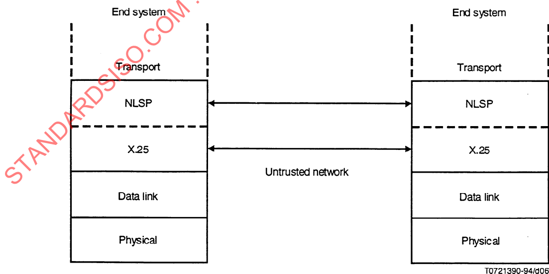
Figure 7 – Illustration of NLSP-CO between end systems
