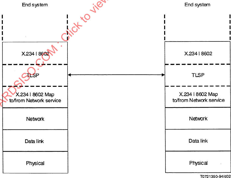
Figure 3 – Illustration of TLSP operating in conjunction with ITU-T Rec. X.234 | ISO/IEC 8602
