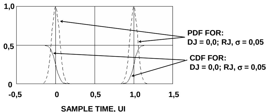
Figure 14 - Jitter eye diagram statistics, linear scale
