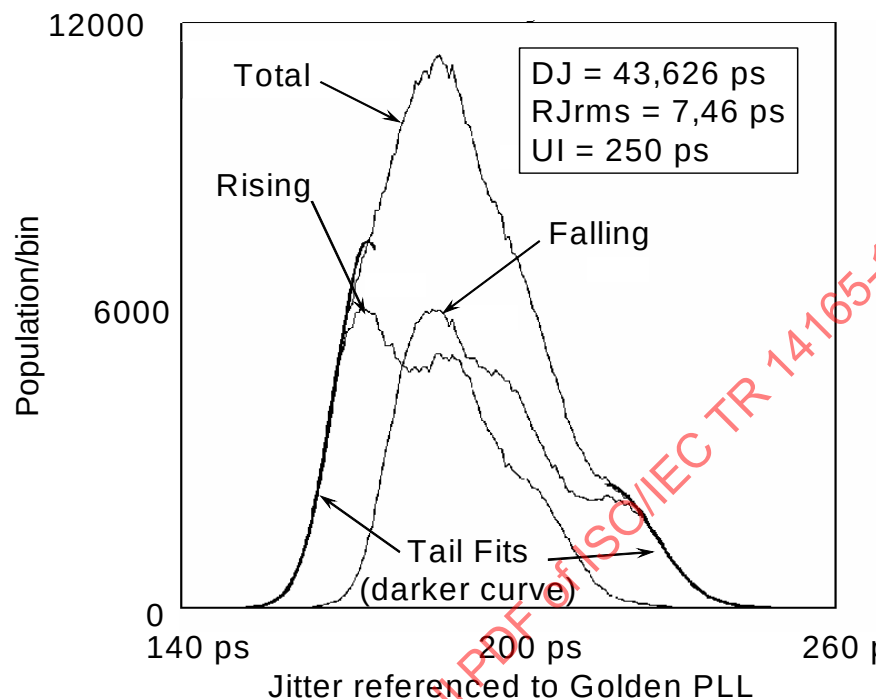
Figure 45 - Total jitter histogram measured with a Golden PLL clock as the reference
