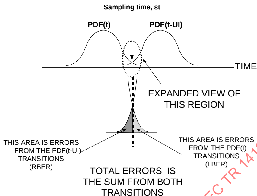
Figure 13 - Probability of signal event errors from adjacent signal transitions
