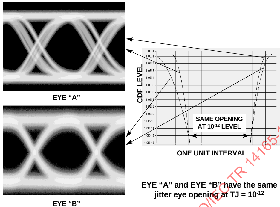
Figure 4 - Waveform eye diagrams from different jitter distributions
