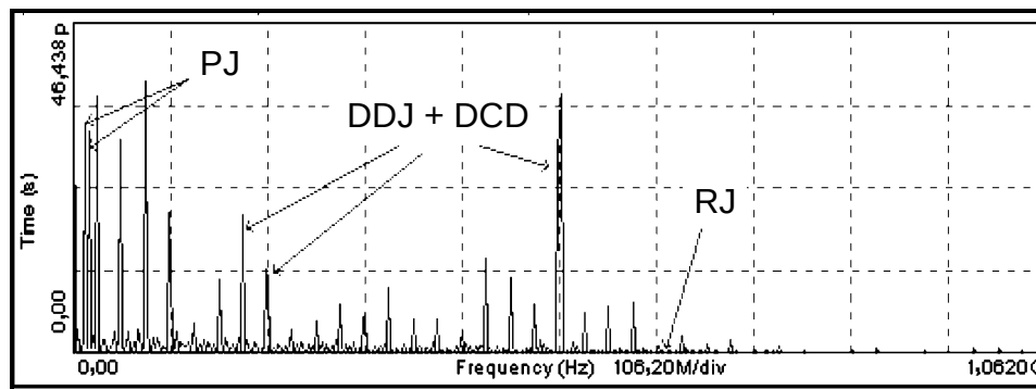
Figure 73 - Frequency spectrum of time interval error (TIE)
