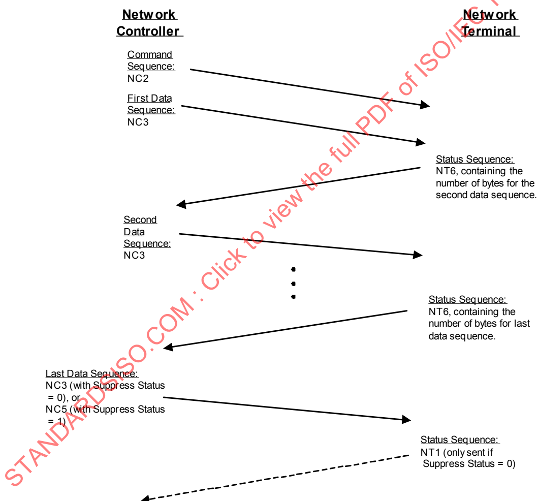
Figure 3 – Network Controller to Network Terminal transfers: NT Burst Size Request = '0'b, Delayed NT Burst Size Request = '1'b
