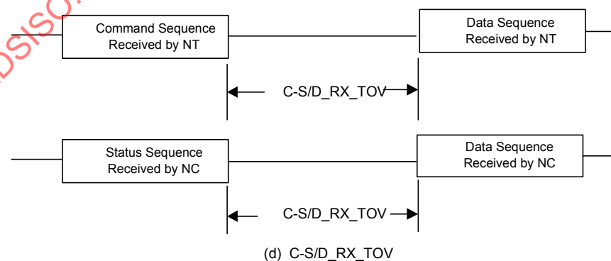
Figure 17 – FC-AE-1553 ULP timers: (a) NT_C/S_TOV and NT_C-D/S_BURST_TOV; (b) NC_C/S_TOV and NC_C-D/S_BURST_TOV; (c) C-S/D_TX_TOV (shown for NC and NT); (d) C-S/D_RX_TOV (shown for NC and NT)
