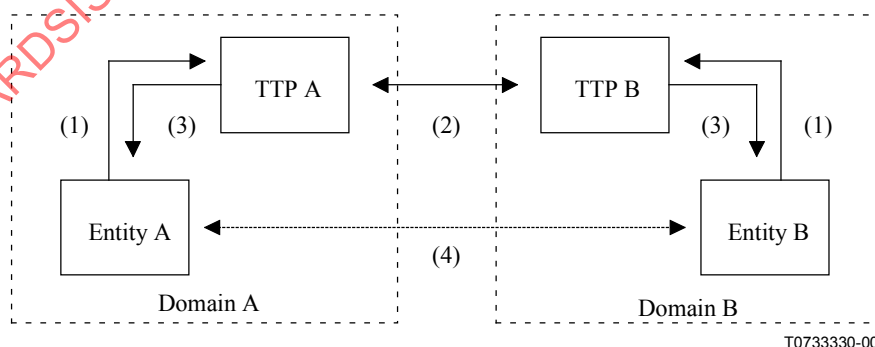
Figure 4 – Interworking of TTPs in Different Domains
