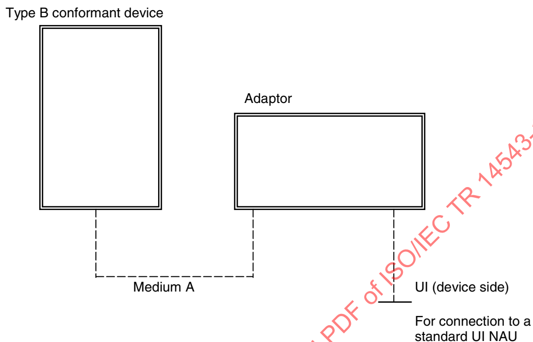
Figure 6 – Type A conformant combination of a type B conformant device and adaptor
