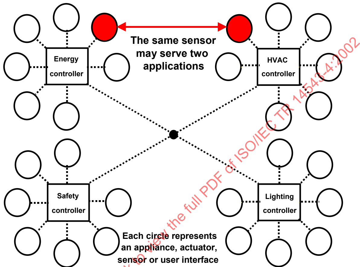
Figure 5 – Interconnecting application domains as peers
