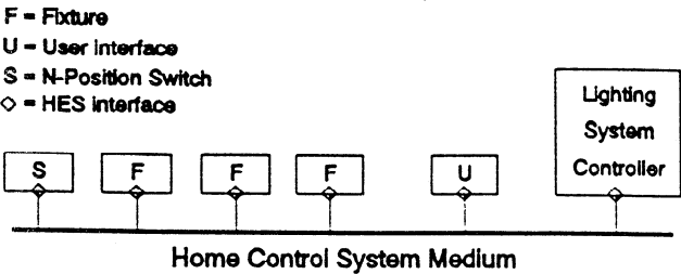
Figure 12: Case 4 — Physical Model
