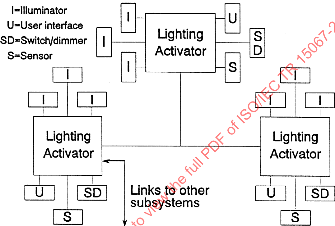
Figure 5: Logical Model of HES Distributed Lighting Control
