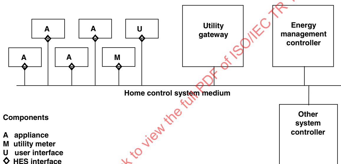
Figure 3 – Physical HES energy management model
