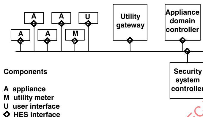
Figure 13 – Case 7: Physical model
