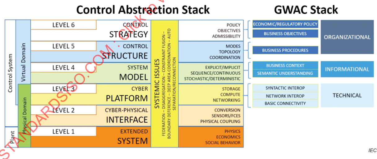
Figure 13 – Integrated Control Abstraction Stack/GWAC Stack model
