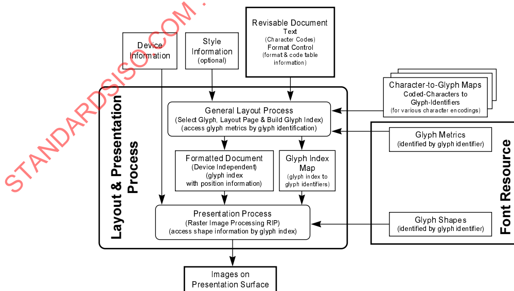
Figure 8 — Font resource model
