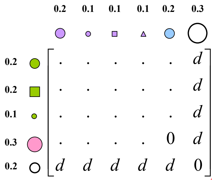
Figure AMD2-4 — Binary-distance matrix from the example in Figure AMD2-3
