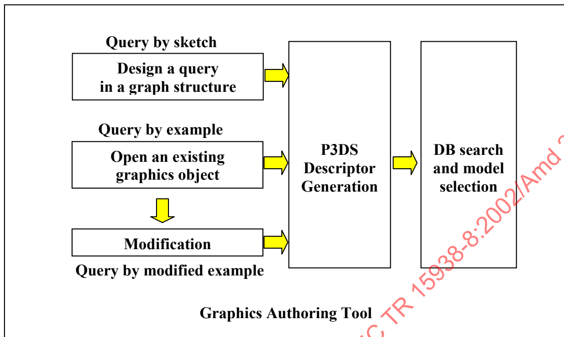
Figure AMD2-5 — The block diagram of the use scenario for the creation of 3D graphic contents
