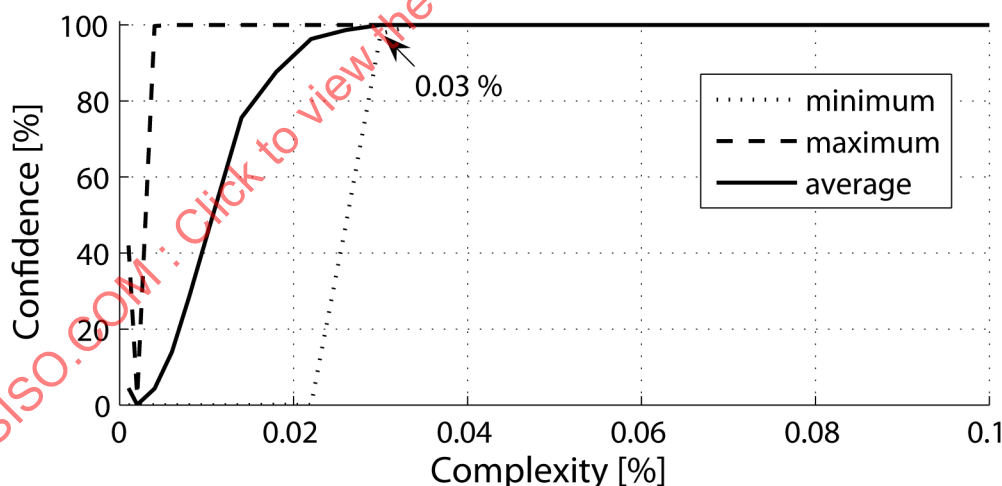
Figure AMD4.6 — Results after classification for MP3 at a sampling rate of 44.1 kHz, confidence vs. conversion complexity for the test set of 100 items.
