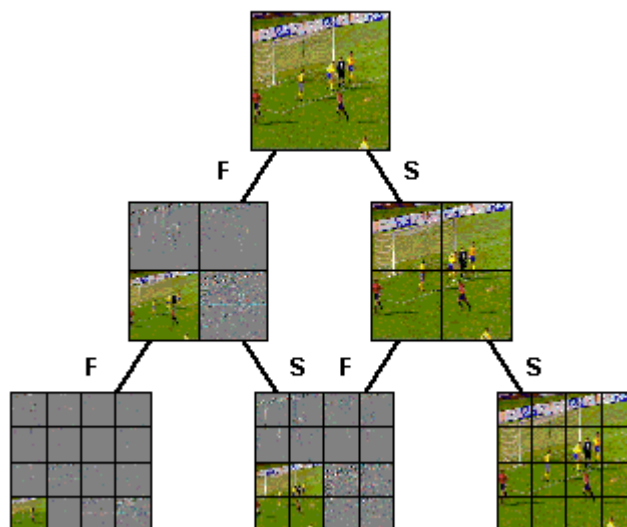
Figure 60 - shows an example Space and Frequency Graph decomposition of an image. The Space and Frequency Graph structure includes node elements that correspond to the different space and frequency views of the image, which consist of views in space (spatial segments), frequency (wavelet subbands), and space and frequency (wavelet subbands of spatial segments). The Space and Frequency Graph structure includes also transition elements that indicate the analysis and synthesis dependencies among the views. For example, in the figure, the "S" transitions indicate spatial decomposition while the "F" transitions indicate frequency or subband decomposition.
