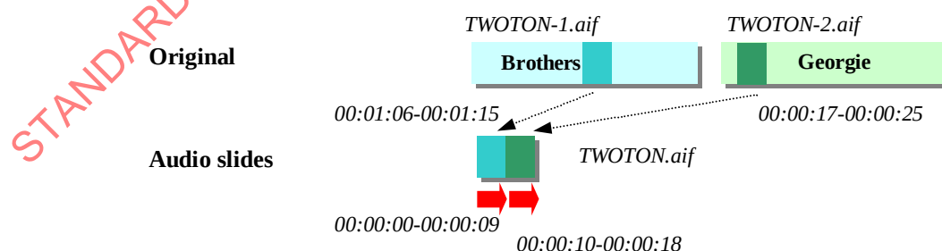
Figure 53 - Example of an audio summary with multiple sources.
