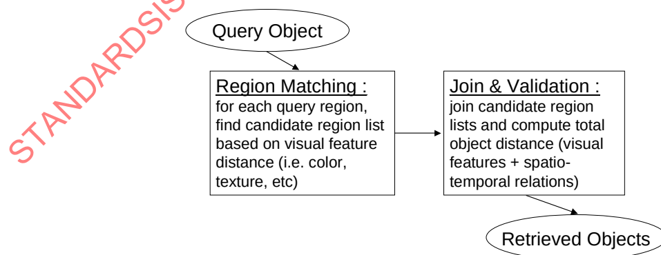
Figure 31 - The video object query model.
