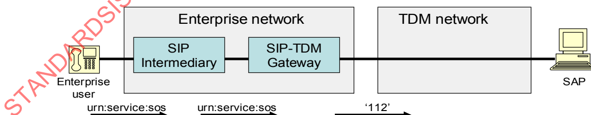
Figure 7 — Example of an emergency call starting with a service URN and submitting a dial string to a TDM network
