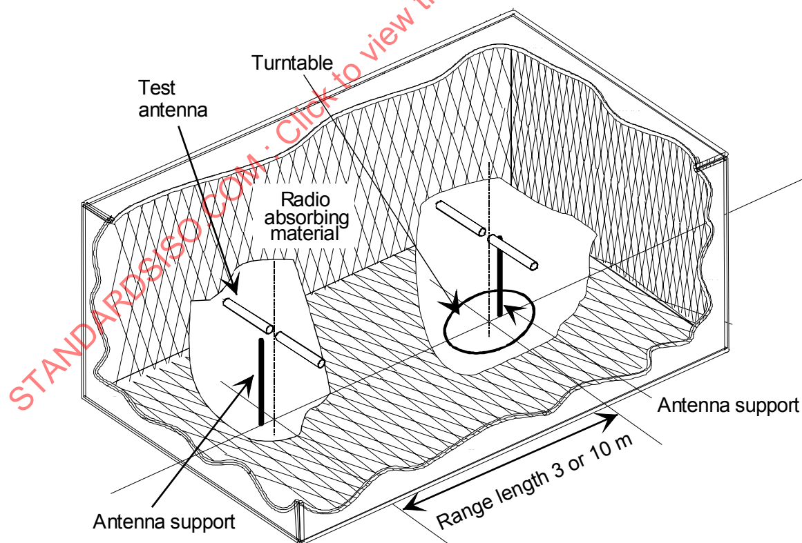
Figure A.1 — A typical anechoic chamber
