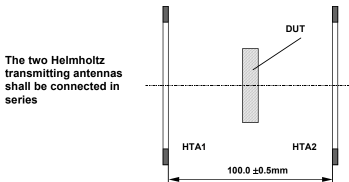
Figure 3 — Helmholtz setup
