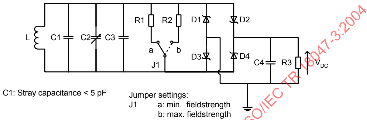
Figure F.1 – Circuit diagram for reference tag
