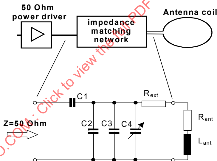
Figure C.3 — Impedance matching network
