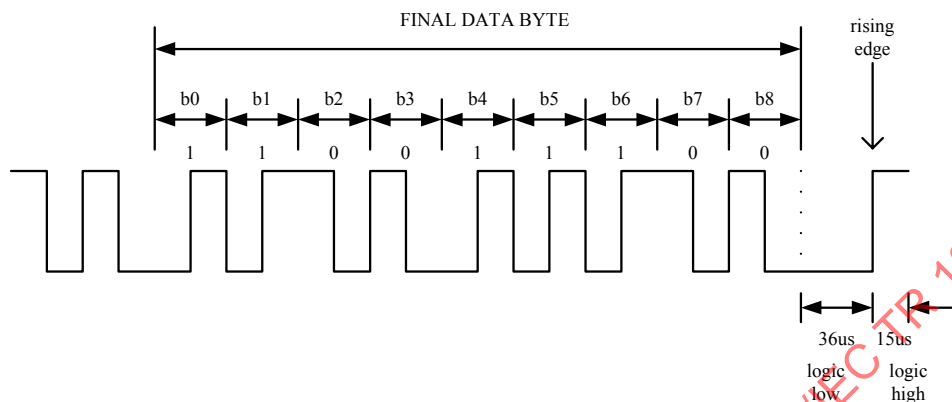
Figure 10 — Final Data Byte Timing
