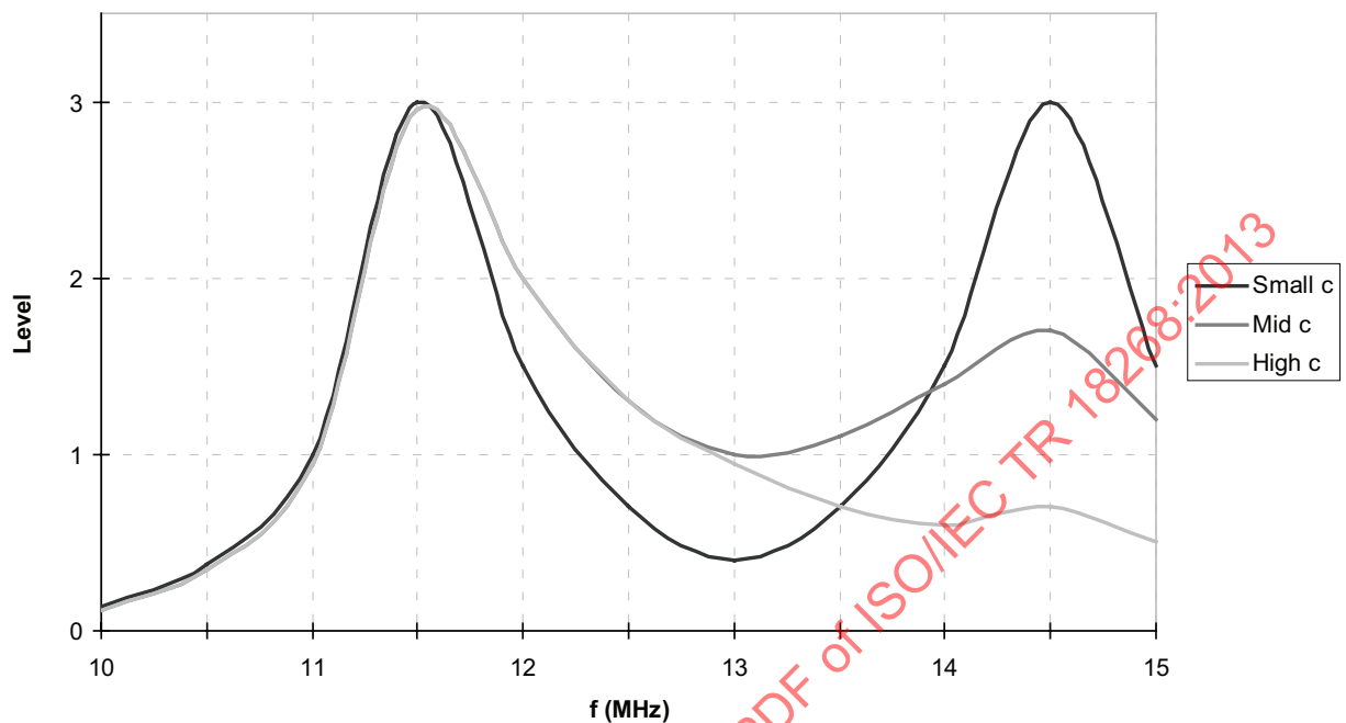
Figure 4 — Effect of capacitance on resonance shift
