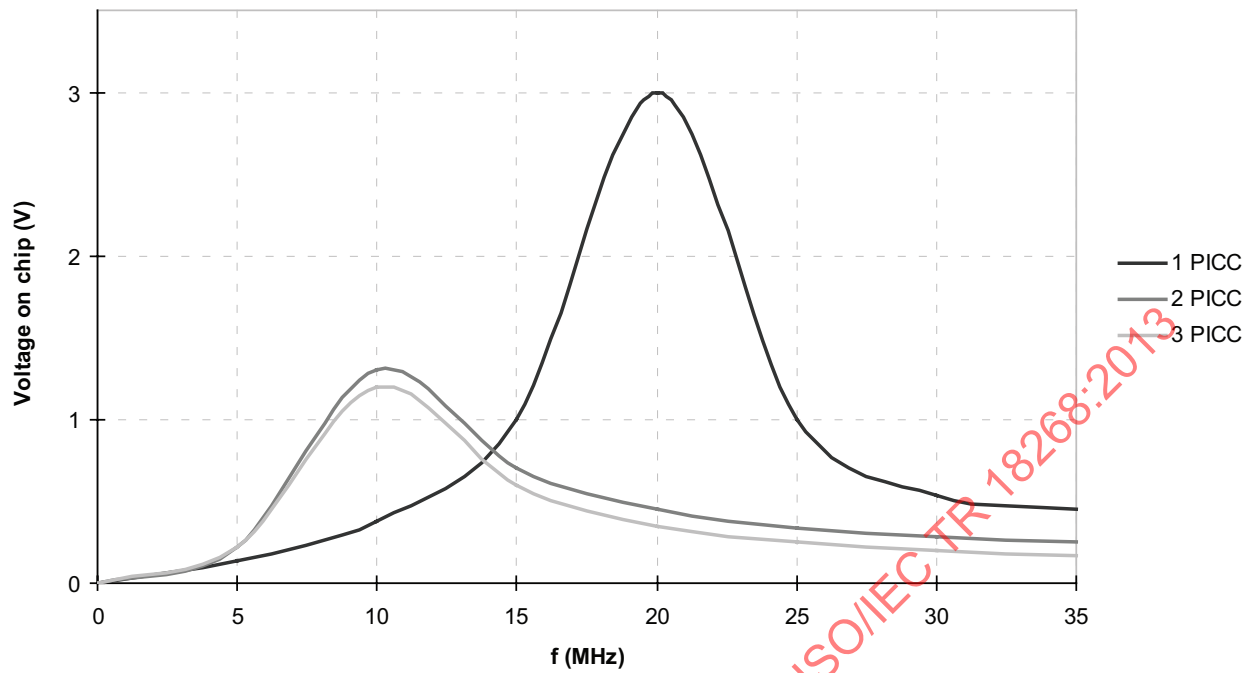
Figure 1 — Power drop and resonance shift
