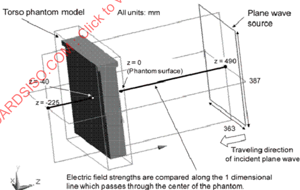
Figure A.7 — Coordinate system for analysis model
