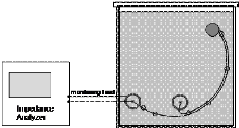
Figure A.16a — measurement setup
