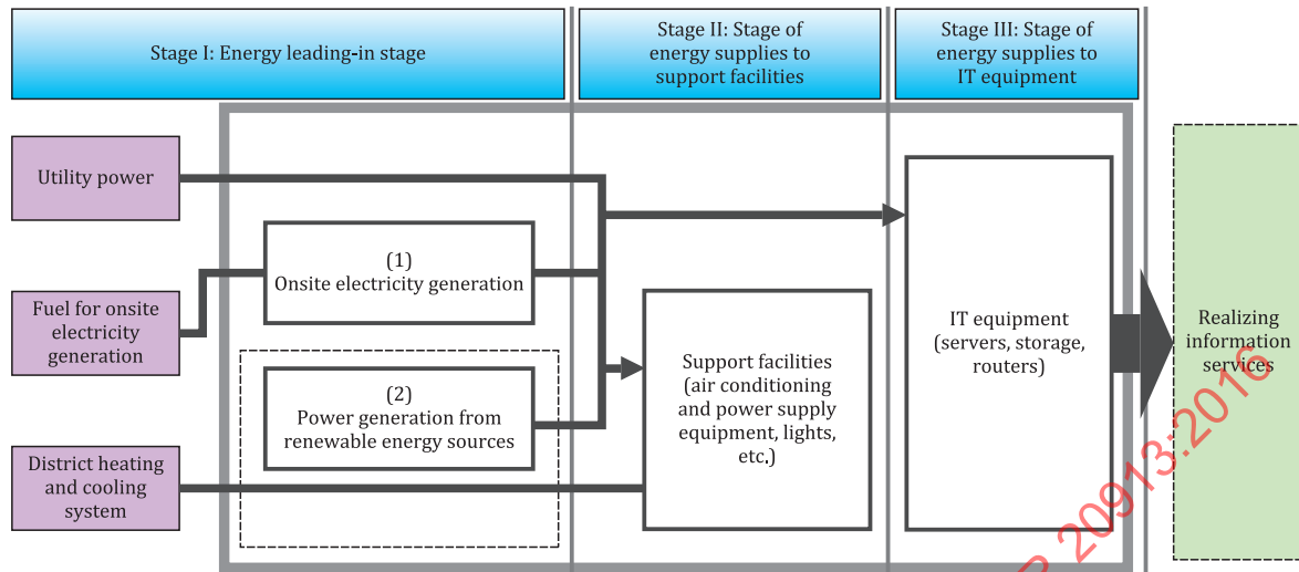
Figure 2 — Flow of energy in a data centre
