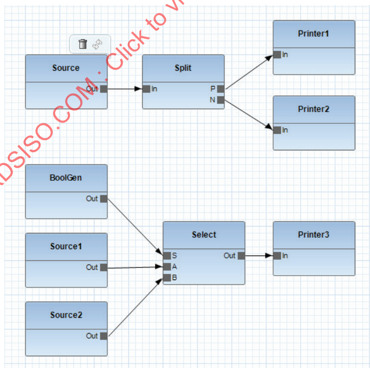
Figure 24 — Network of simple actors to explain guarded actions
