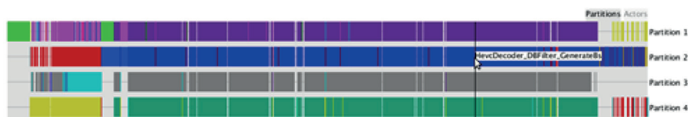
Figure 39 — Per-partition chronological trace for an HEVC decoder specification
