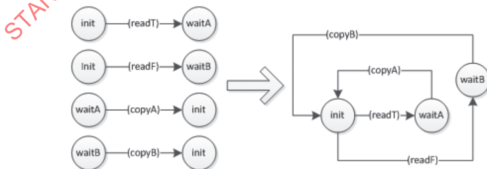
Figure 26 — State transitions and the equivalent finite state machine
