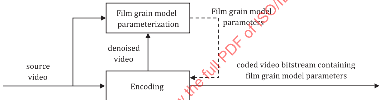
Figure 5 — Use of film grain modelling technologies with an encoder to denoise source video
