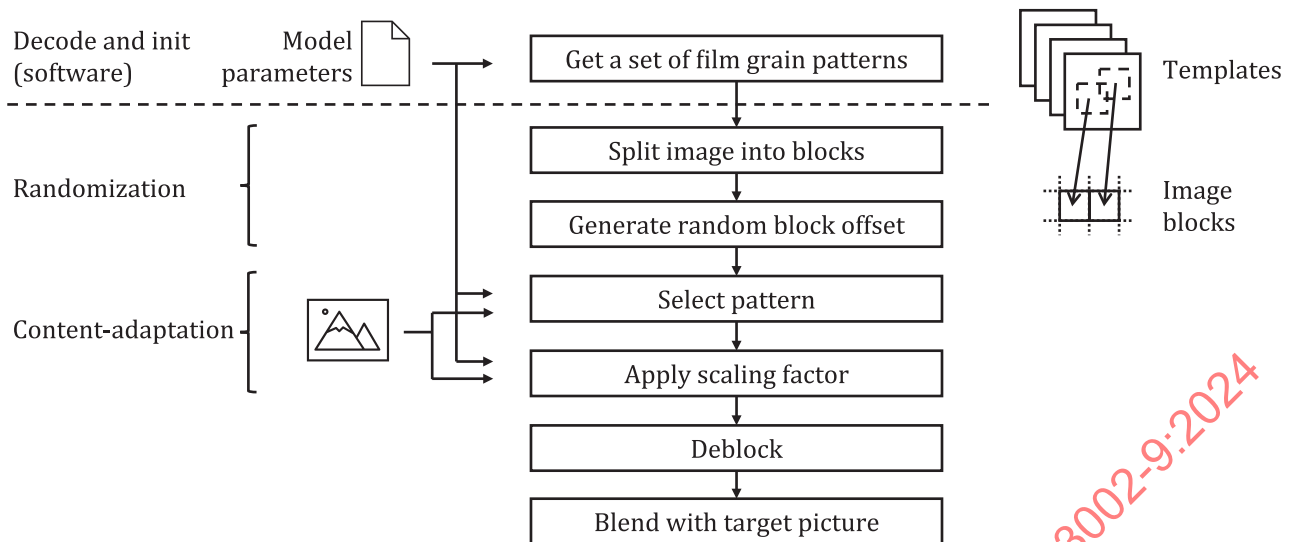
Figure 8 — Template-based film grain synthesis workflow
