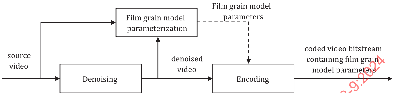
Figure 4 — Use of film grain modelling technologies with a denoising pre-processing stage
