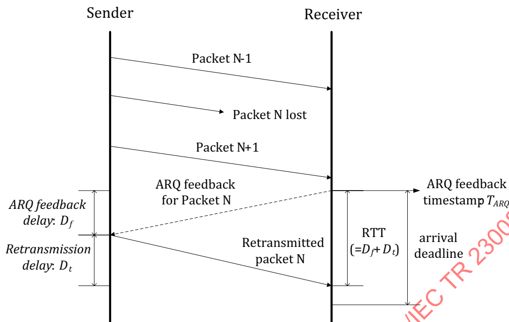
Figure 24 — Operation of the arrival-deadline constrained ARQ
