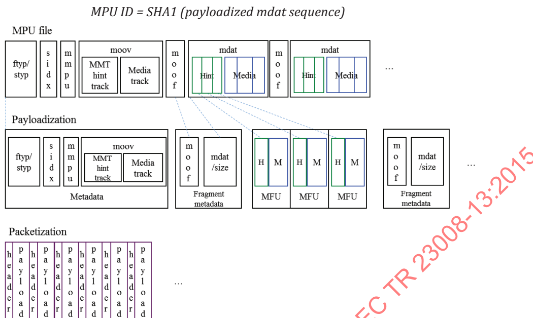
Figure 44 — Payloadized format
