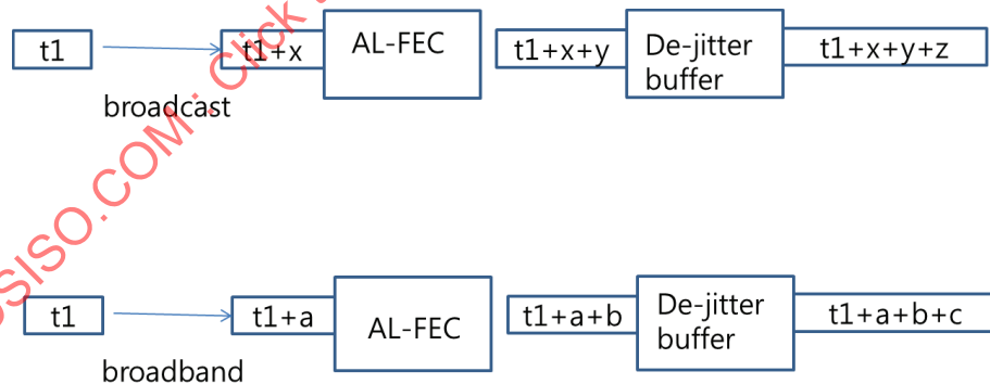
Figure 20 — HRBM buffers
