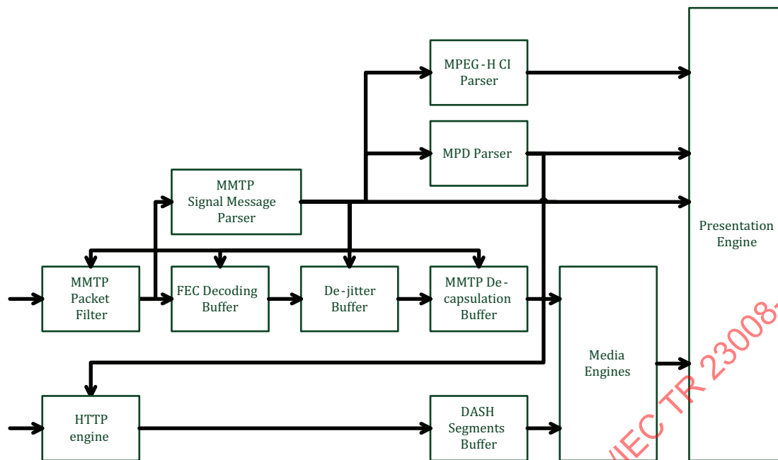
Figure 41 — Conceptual architecture of hybrid service client
