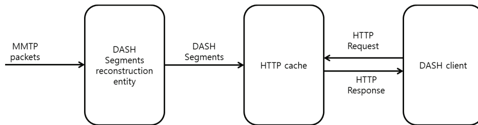
Figure 38 — Client with HTTP cache
