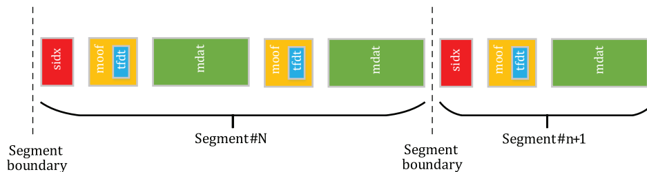
Figure 37 — Segment boundary detection
