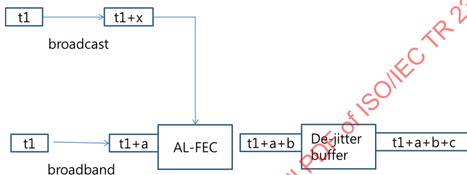
Figure 36 — Jitter reducing mechanism by broadcasting repair
