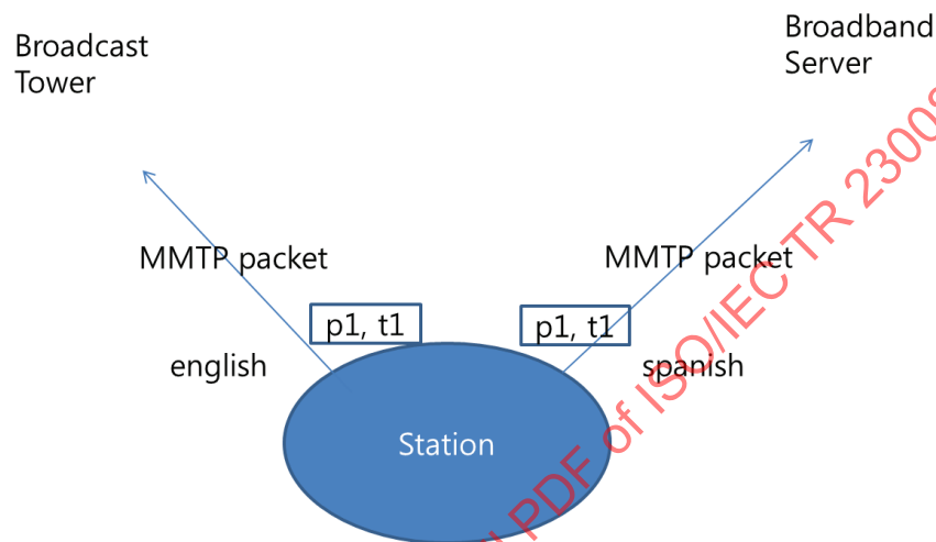
Figure 34 — Hybrid service for primary and secondary audios
