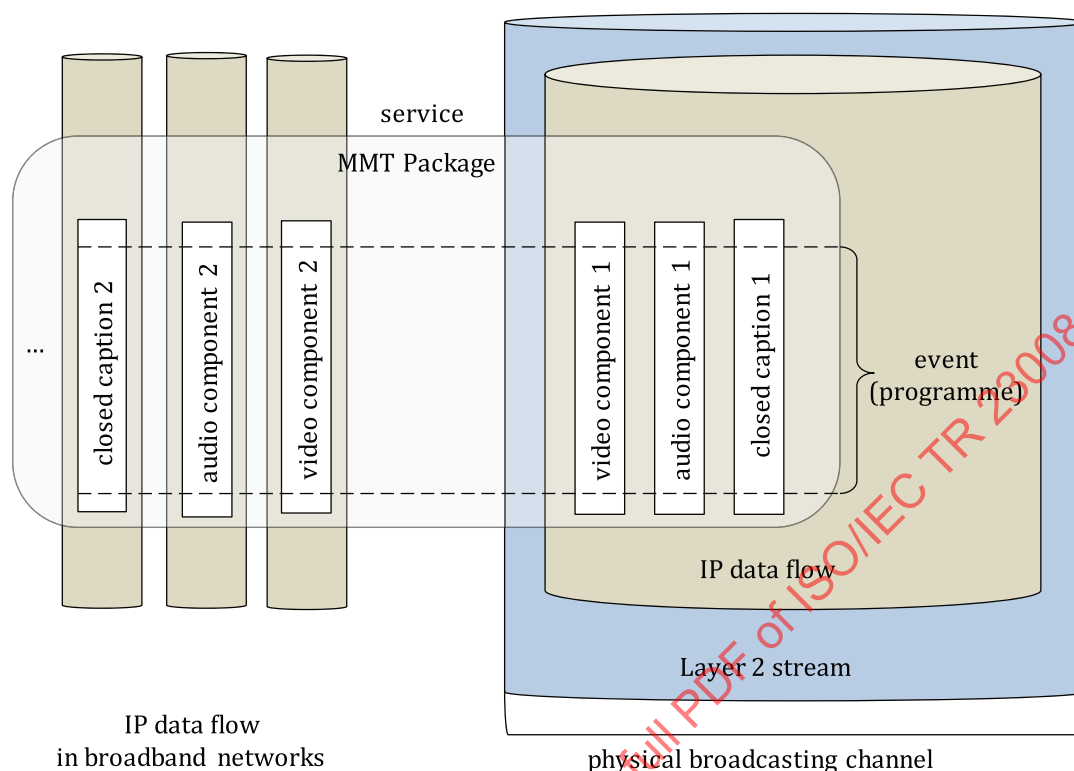
Figure 58 — Service configuration over both broadcasting channels and broadband networks
