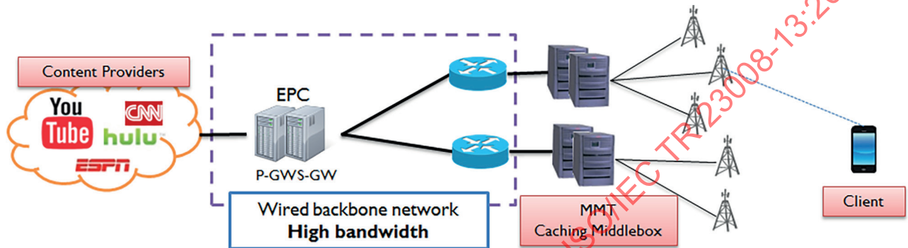
Figure 45 — Overview of an MMT caching middlebox
