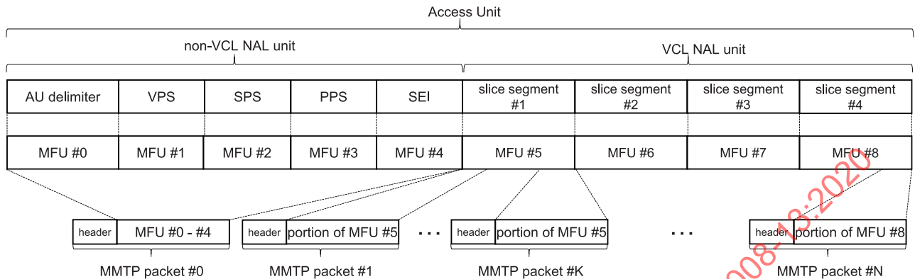
Figure 53 — Overview of packetization of NAL units of HEVC streams
