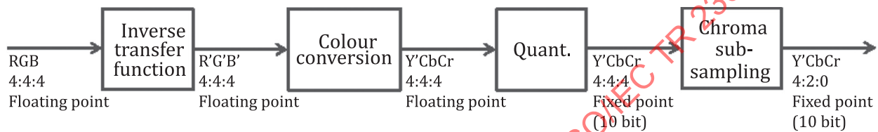
Figure 2 — Conventional pre-encoding process system diagram
