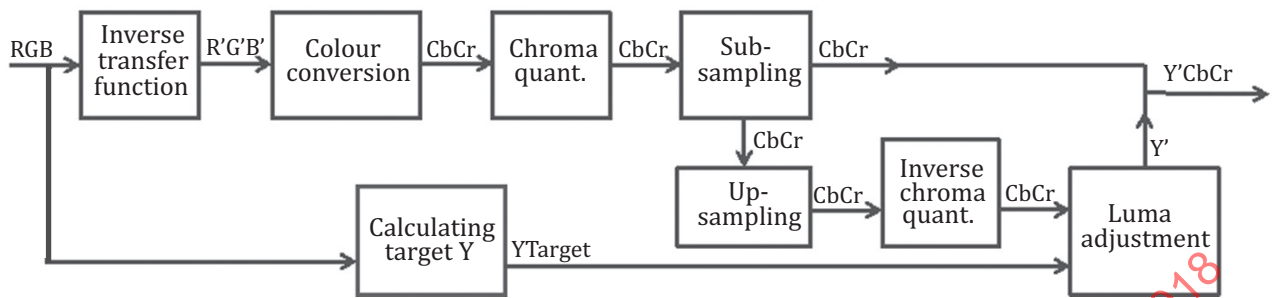
Figure 7 — Example schematic diagram of a closed loop pre-encoding conversion system
