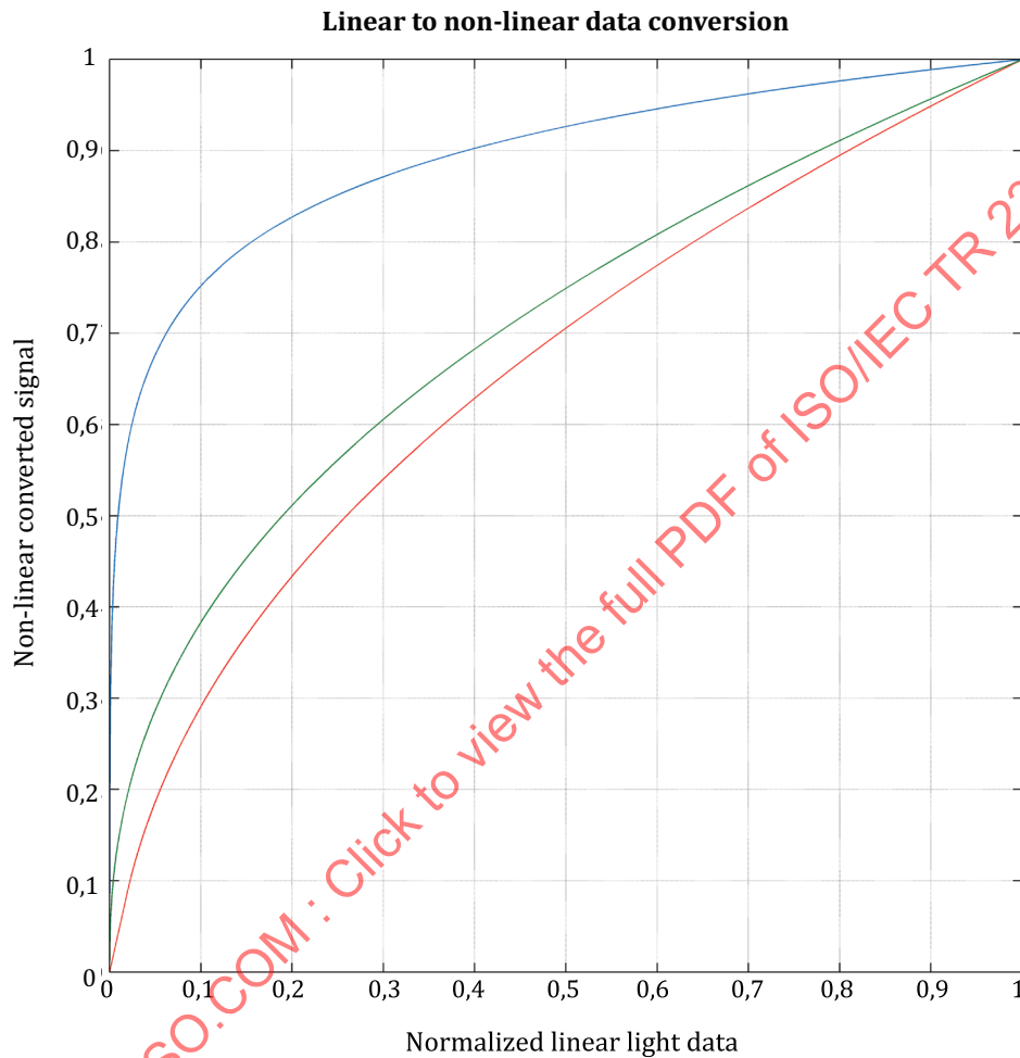
Figure 3 — Inverse of the PQ EOTF (top curve), inverse of the Rec. ITU-R BT.1886 EOTF (middle curve), and the Rec. ITU-R BT.709 OETF (bottom curve)
