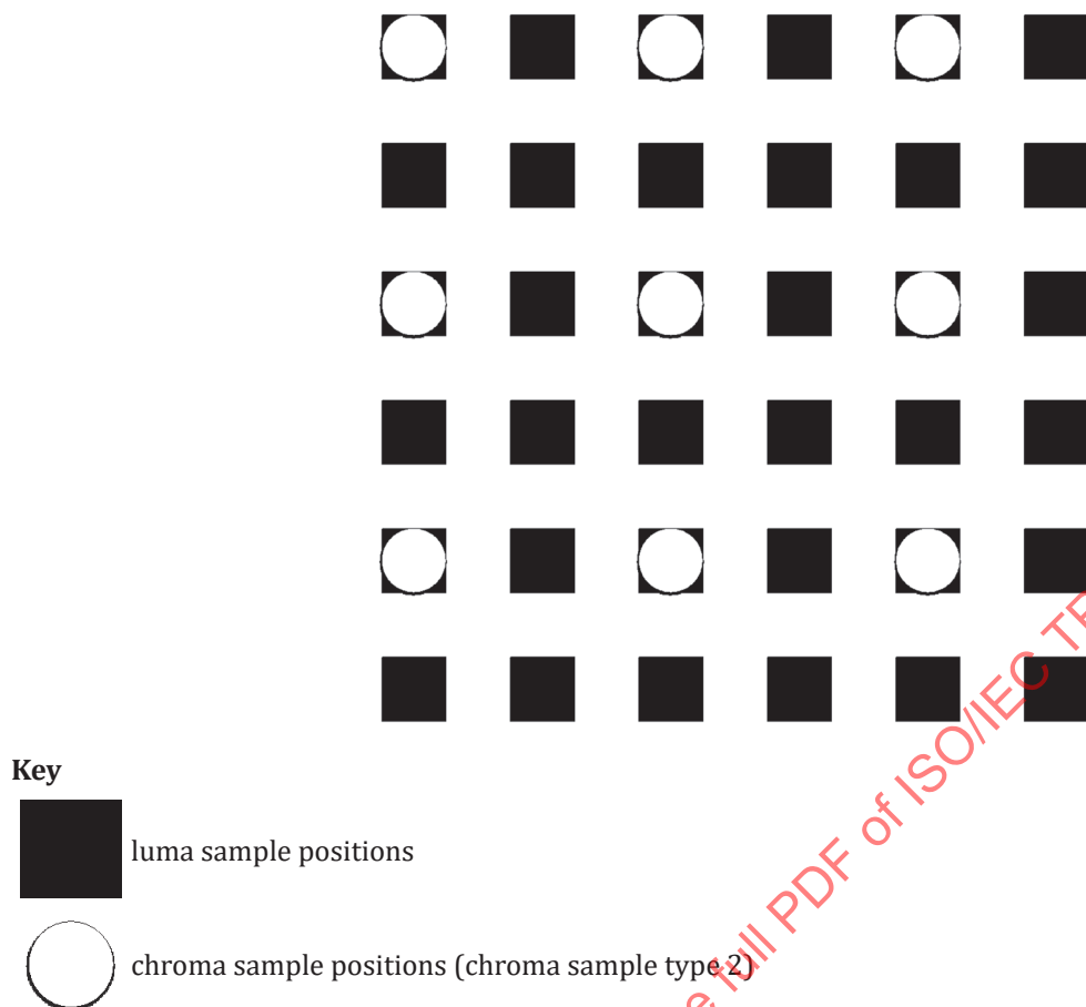
Figure 4 — Chroma and luma sample location relationship
