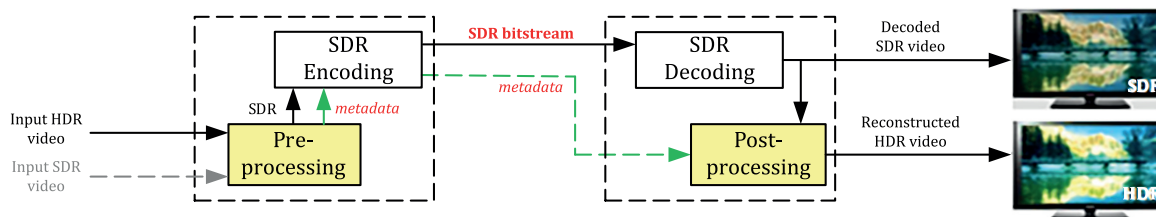
Figure 8 — Bitstream SDR backward compatibility using single layer coding system
