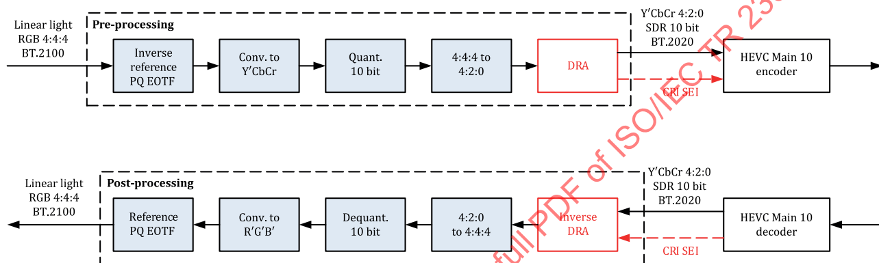
Figure 9 — Pre-processing (top) and post-processing (down) for conversion from SDR/Rec. ITU-R BT.2020-2 to HDR/Rec. ITU-R BT.2100-1 with CRI applied in Y'CbCr 4:2:0 domain
