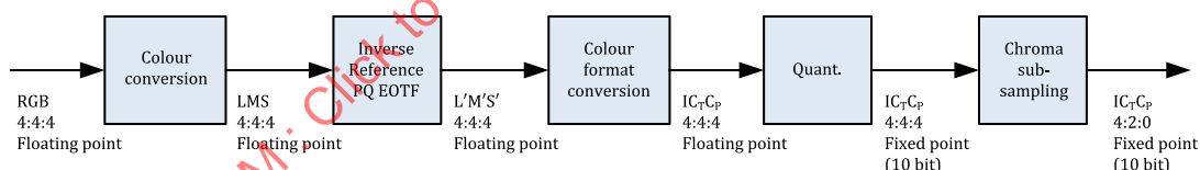
Figure 3 — Conventional PQ IC T C P pre-encoding process system diagram
