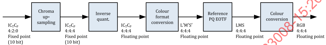
Figure 5 — Conventional PQ IC T C P post-decoding process system diagram
