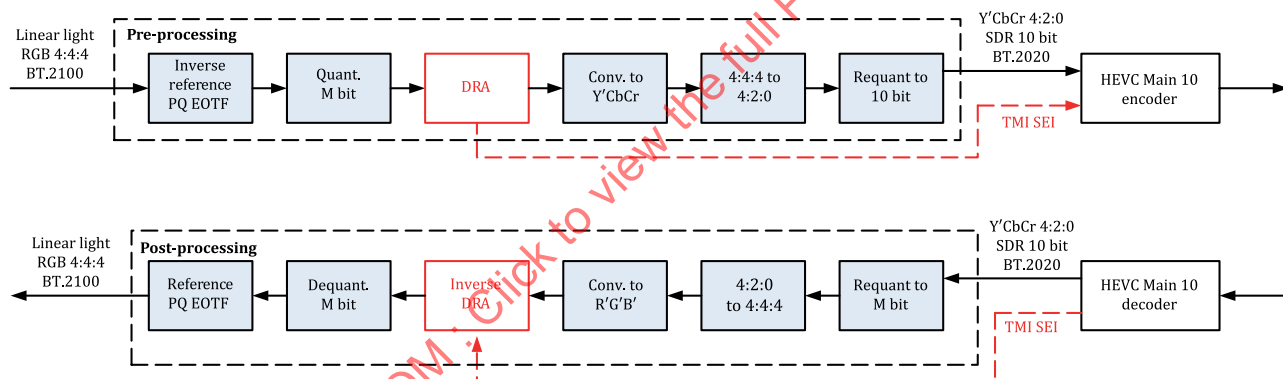
Figure 11 — Pre-processing (top) and post-processing (down) for conversion from SDR/Rec. ITU-R BT.2020-2 to HDR/Rec. ITU-R BT.2100-1 with TMI applied in RGB 4:4:4 domain
