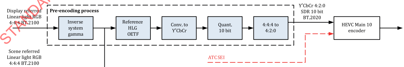
Figure 6 — Conventional HLG Y'CbCr pre-encoding process system diagram
