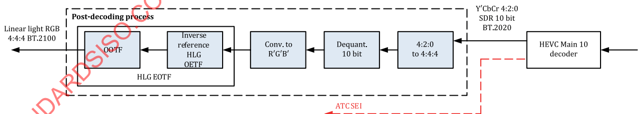
Figure 7 — Conventional HLG Y'CbCr post-decoding process system diagram
