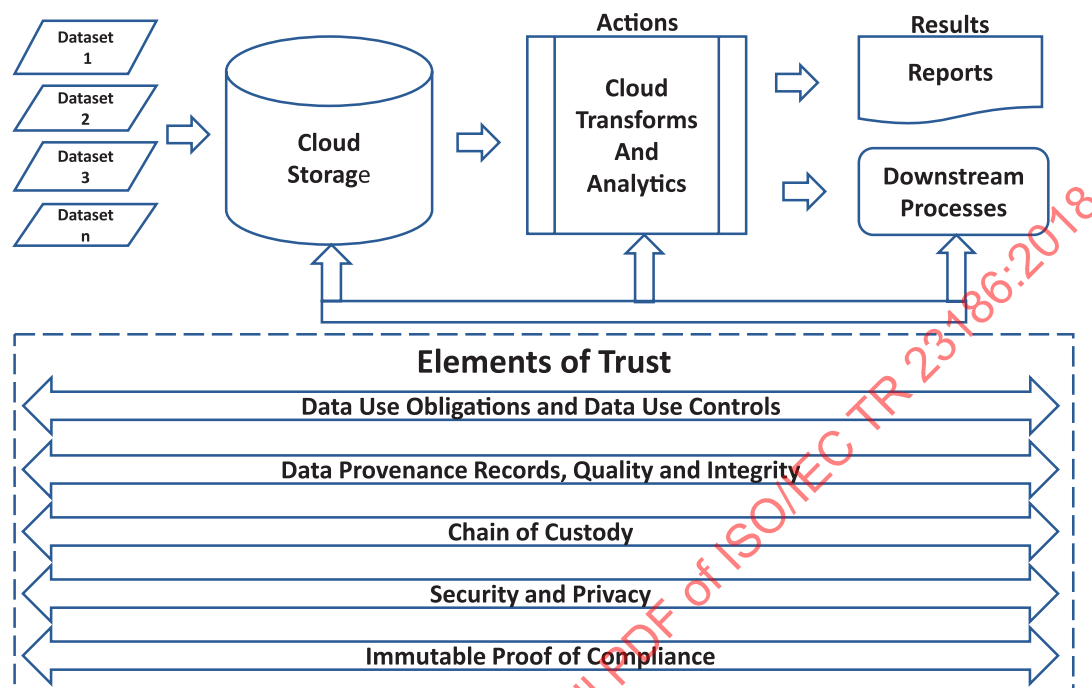
Figure 2 — Framework for trusted cloud processing of multi-sourced data
