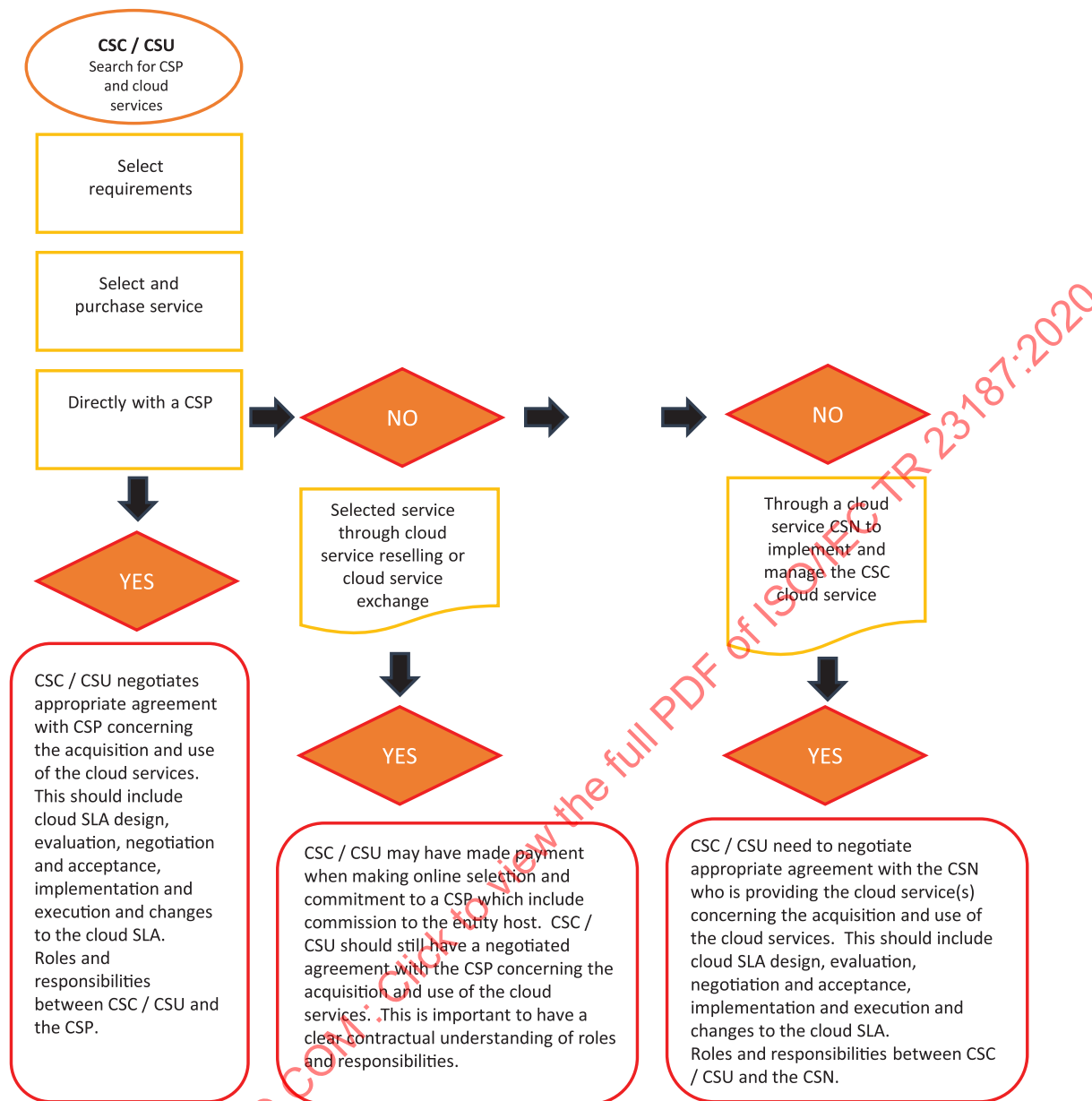
Figure 6 — Scenarios and SLAs
