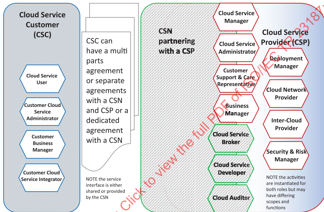
Figure 8 — CSC using a managed service
