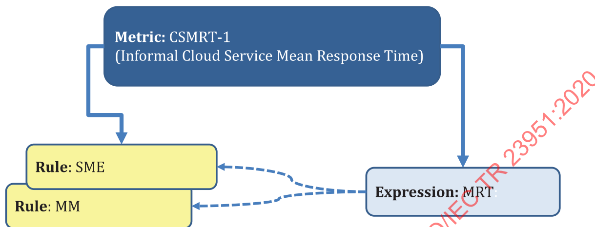
Figure 2 — The elements of the mean response time CSMRT-1 metric
