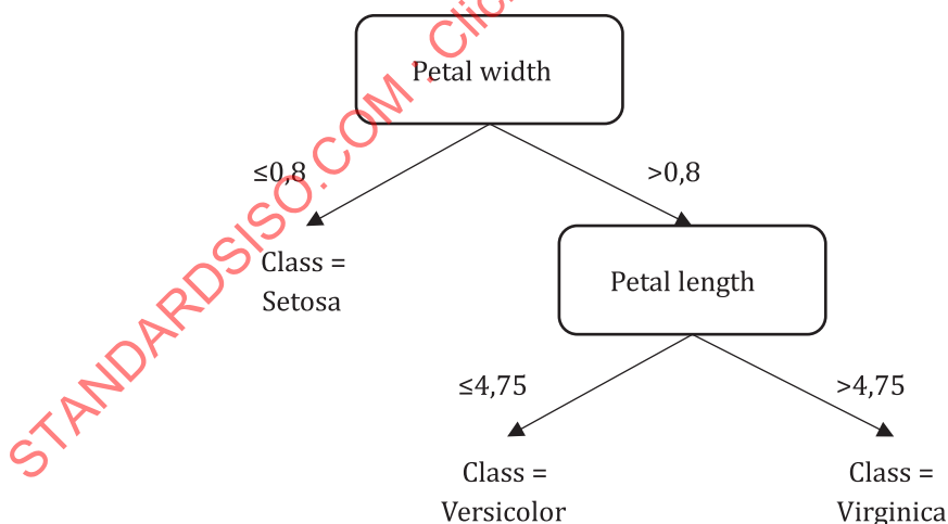
Figure 4 — Example of a decision tree
