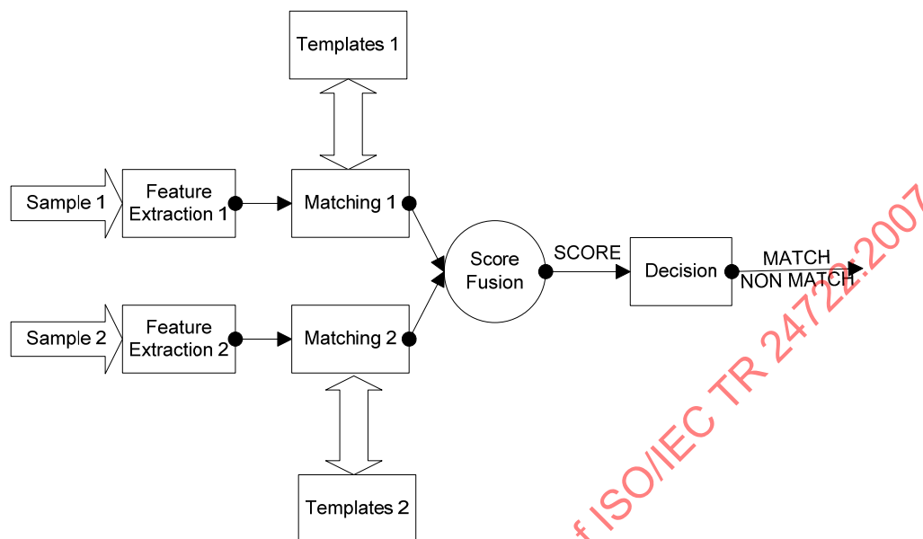
b) Score-level fusion
