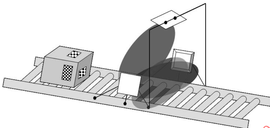
Figure 17 — Partially oriented carton with 3 antennas biased to front & top reads
