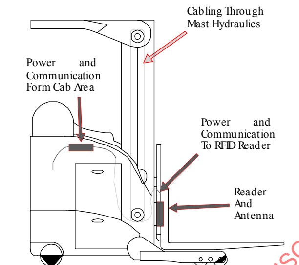
Figure 20 — Forklift mounted reader
