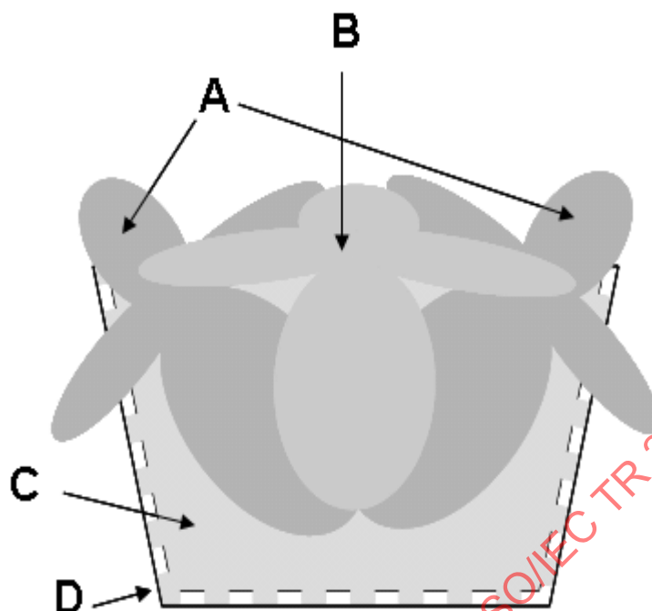
Figure 11 — Three-antenna pattern overlap
