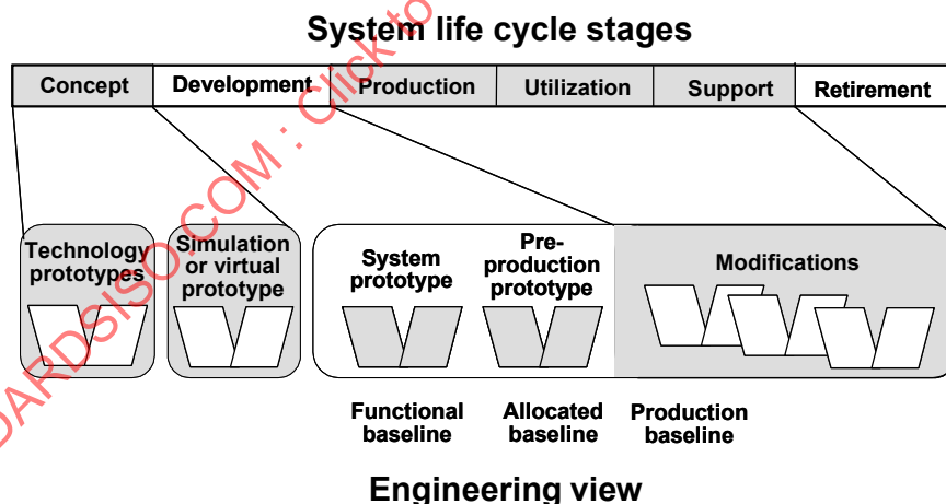
Figure 24 — Engineering view with engineering "Vee" models
