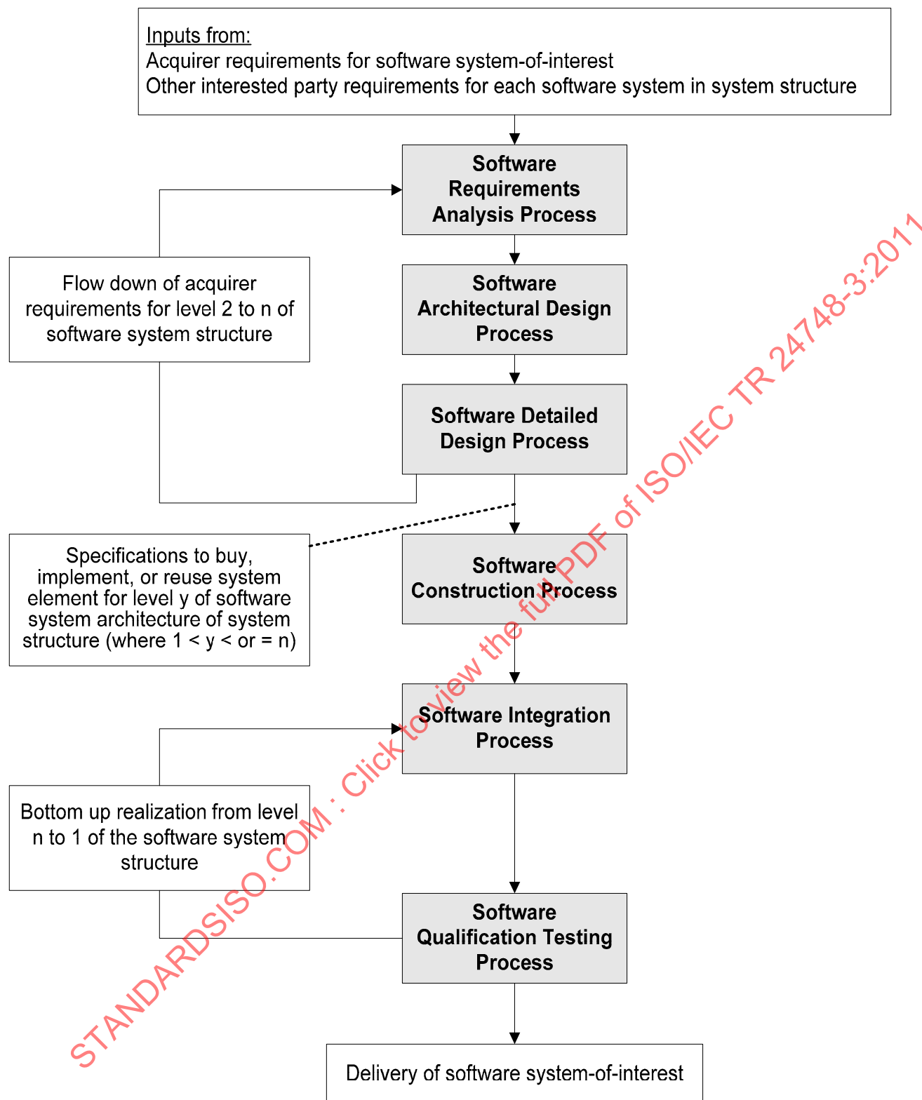
Figure 21 — Application of the Software Implementation Processes to engineer a software system-of-interest
