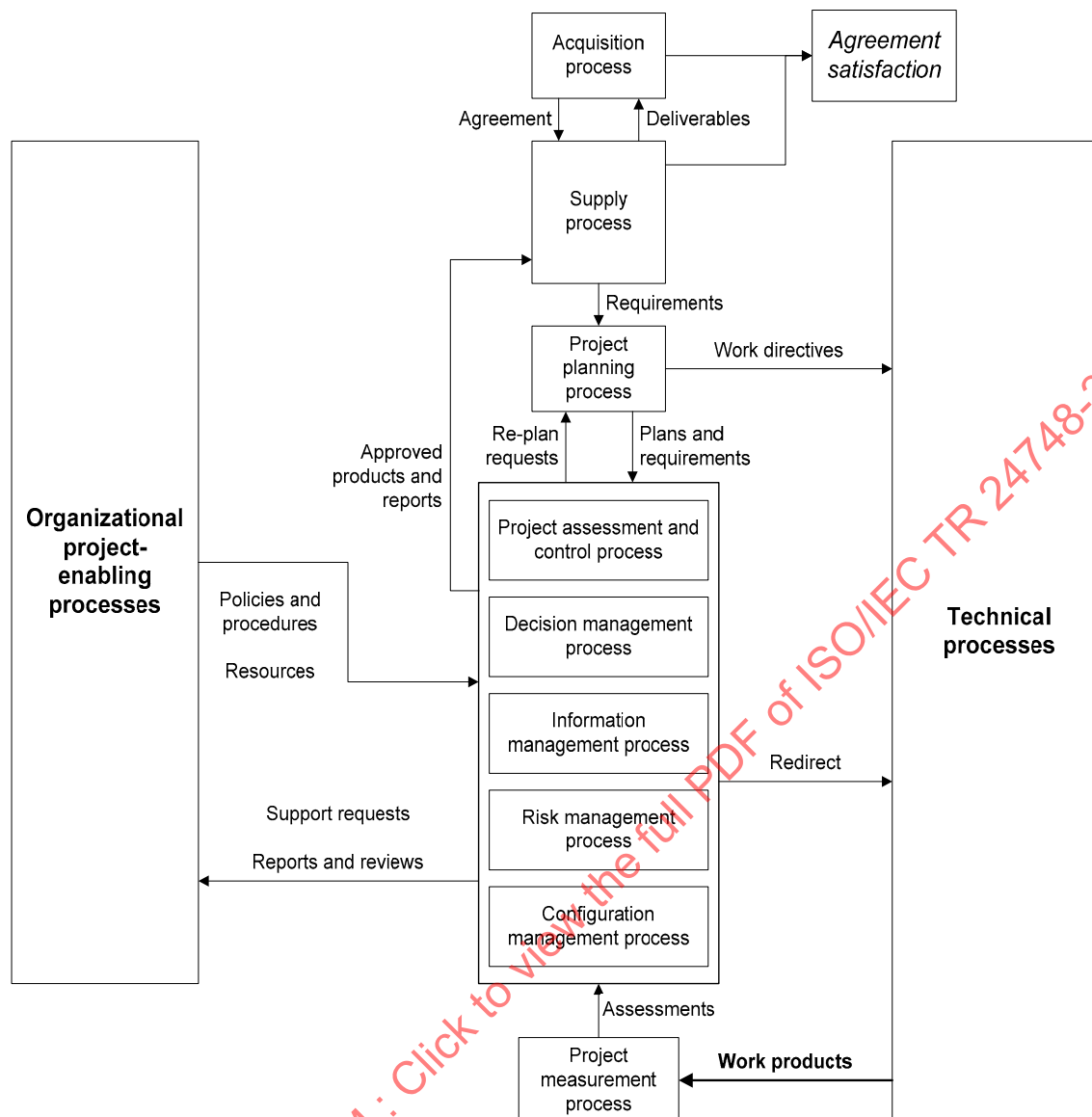
Figure 18 — Application of processes to satisfy an agreement
