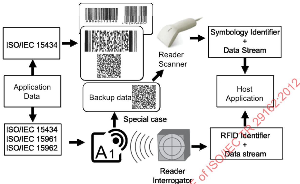
Figure 3 — Operation of data carrier identifiers
