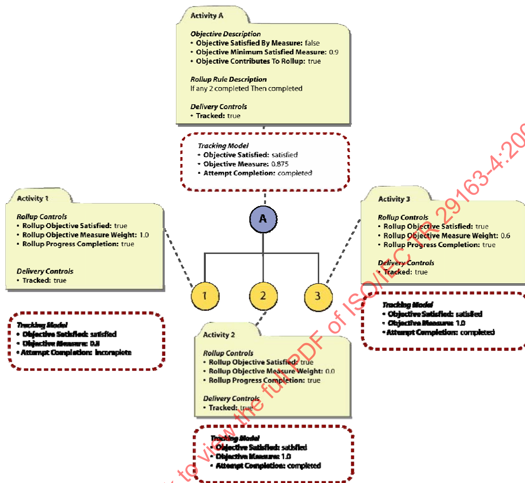
Figure 4.6.5a: Activity Progress Status Rollup Using Rules
