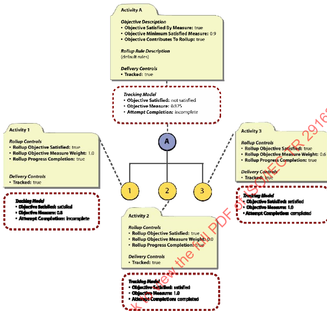
Figure 4.6.5b: Activity Progress Rollup Using Default Rule
