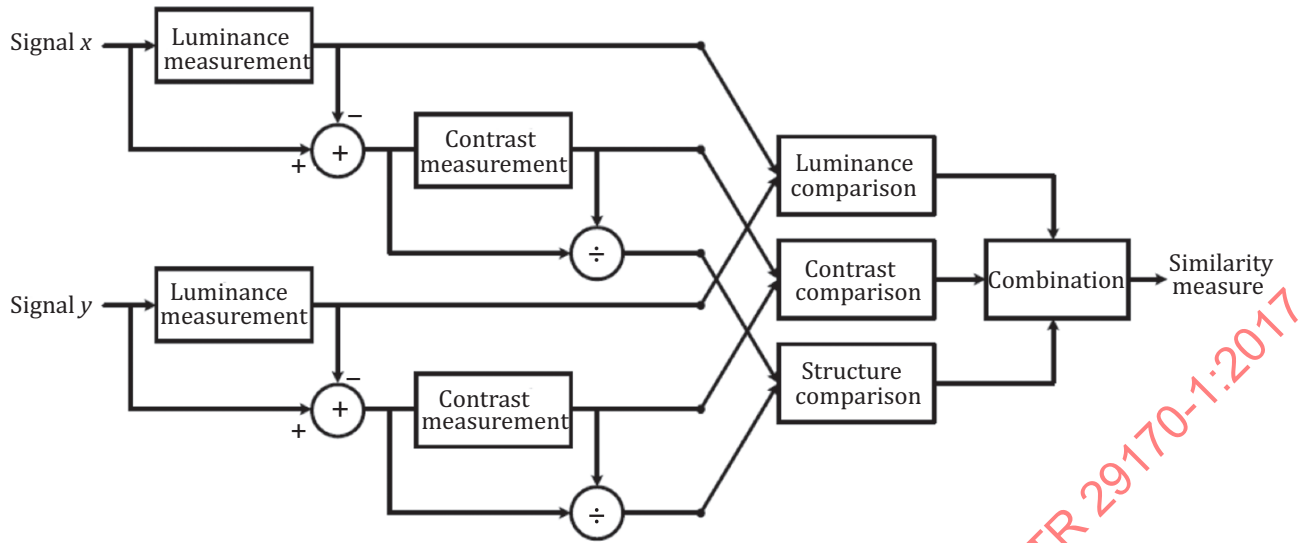
Figure B.1 — Flowchart of the SSIM metric
