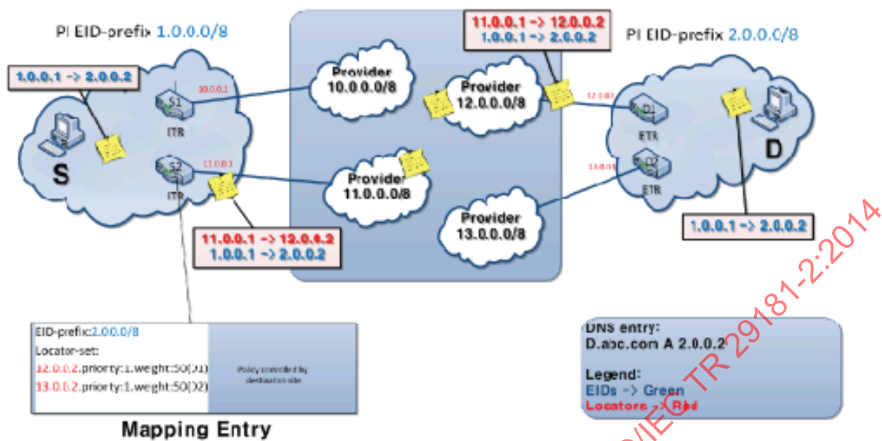
Figure B.2 — Information flow in LISP using EID and RLOC
