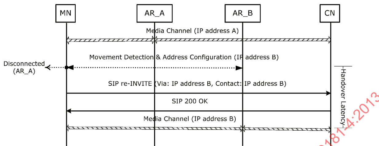
Figure A.2 — Information flow of SIP handover
