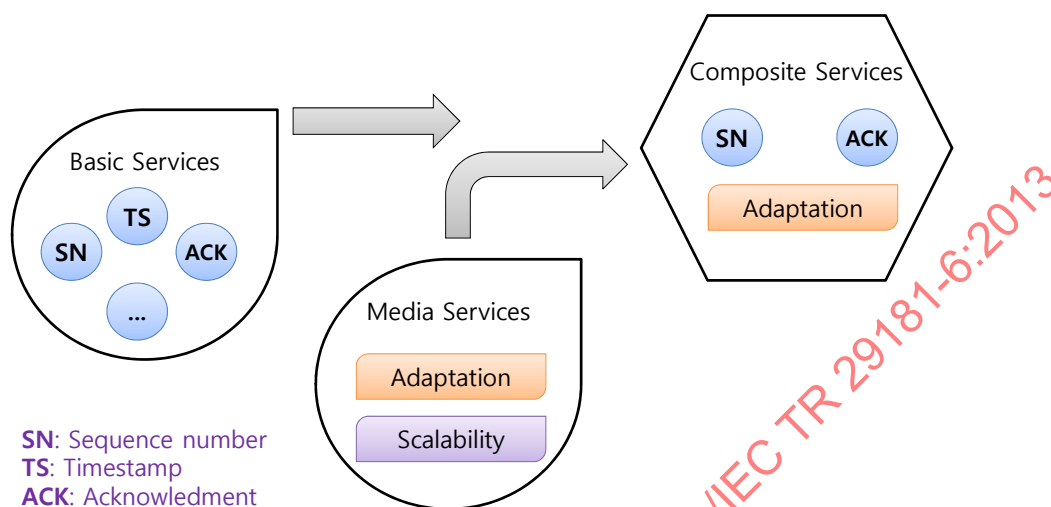
Figure 5 — Basic services and composite services
